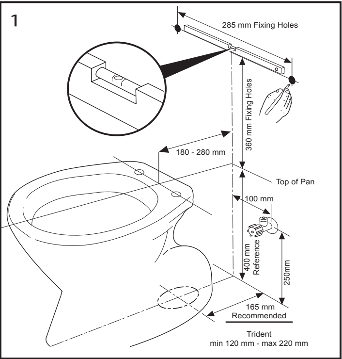
Check that the pan is installed within dimensional tolerances. Mark out the fixing holes for the cistern on the wall. Make sure they are level.
